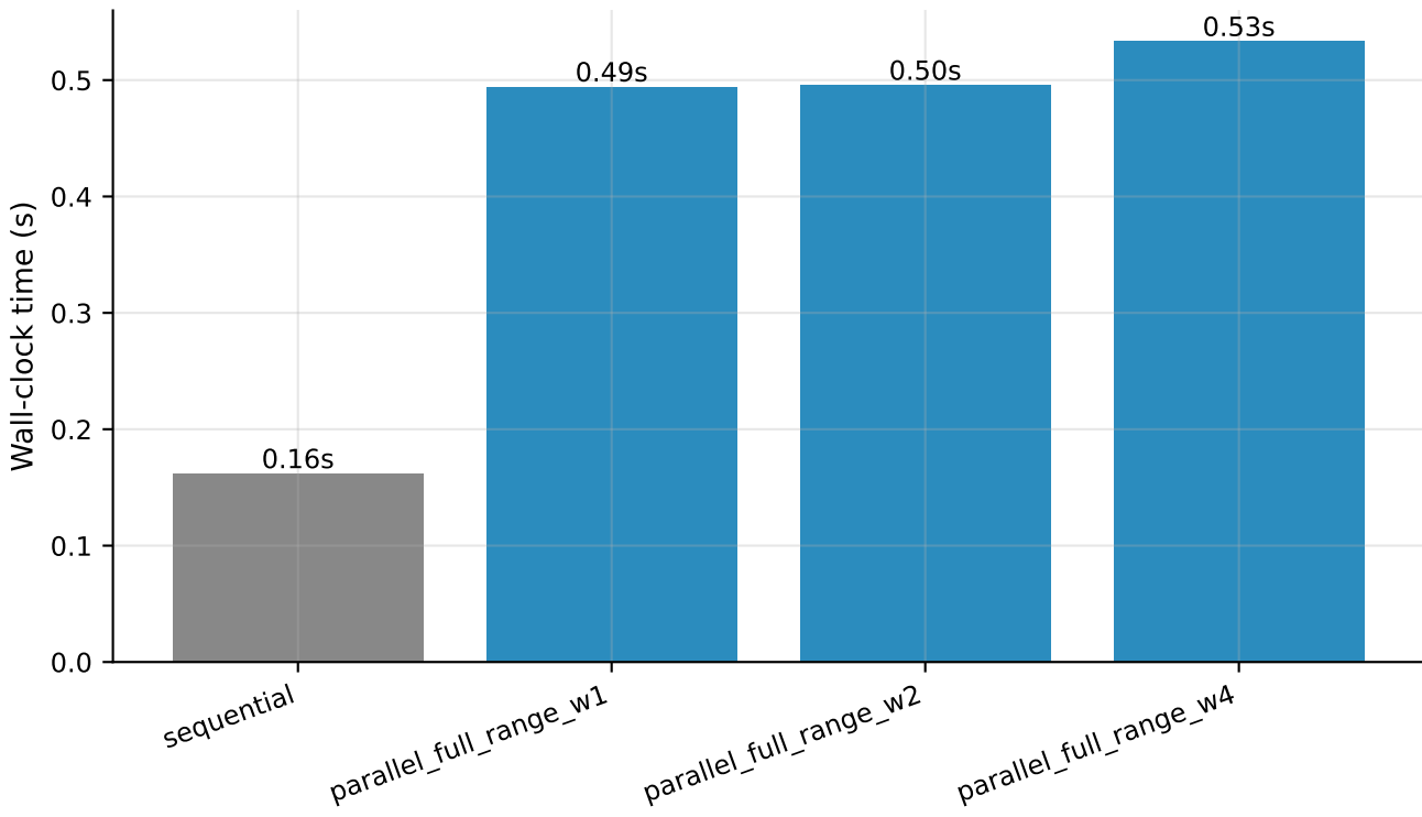
Group A - Sequential vs Parallel PageRank
